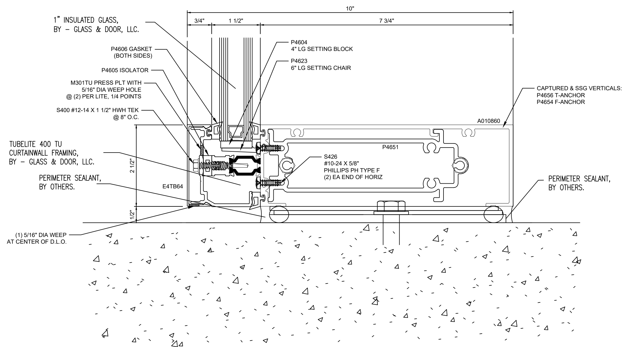
3 SECTION VIEW ● CURTAINWALL SILL
