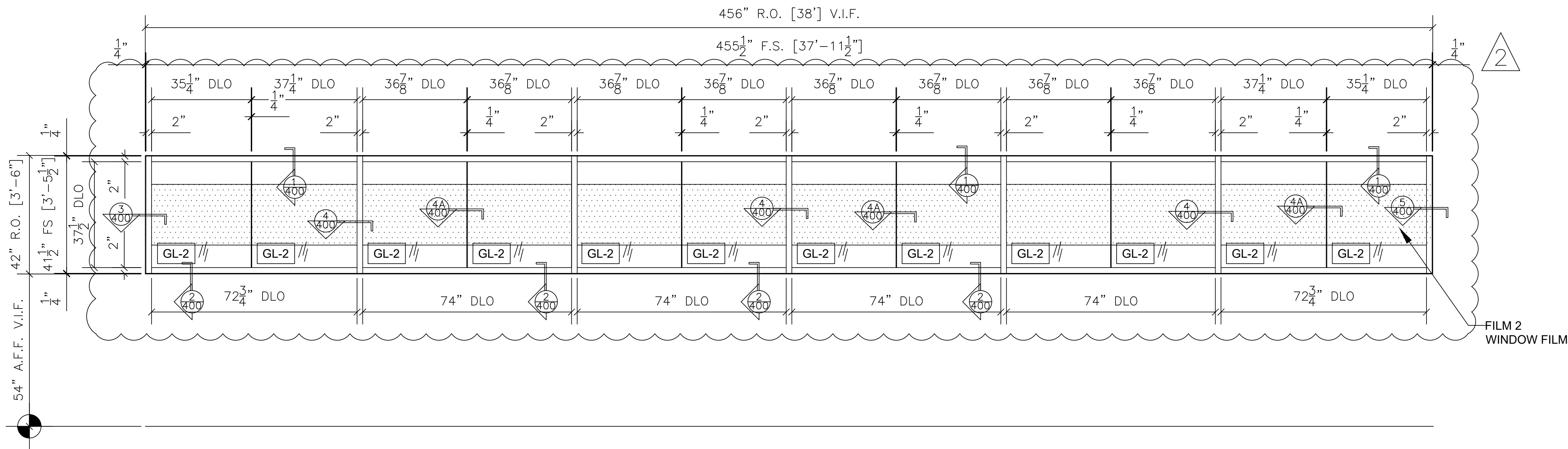
6 WINDOW FRAMING ELEVATION QTY LOCATION 1 NORTH ARTERY 123 1 TOTAL TUBELITE E14000 INTERIOR STOREFRONT ARCH. REF.: SIM. 4/A3.31
