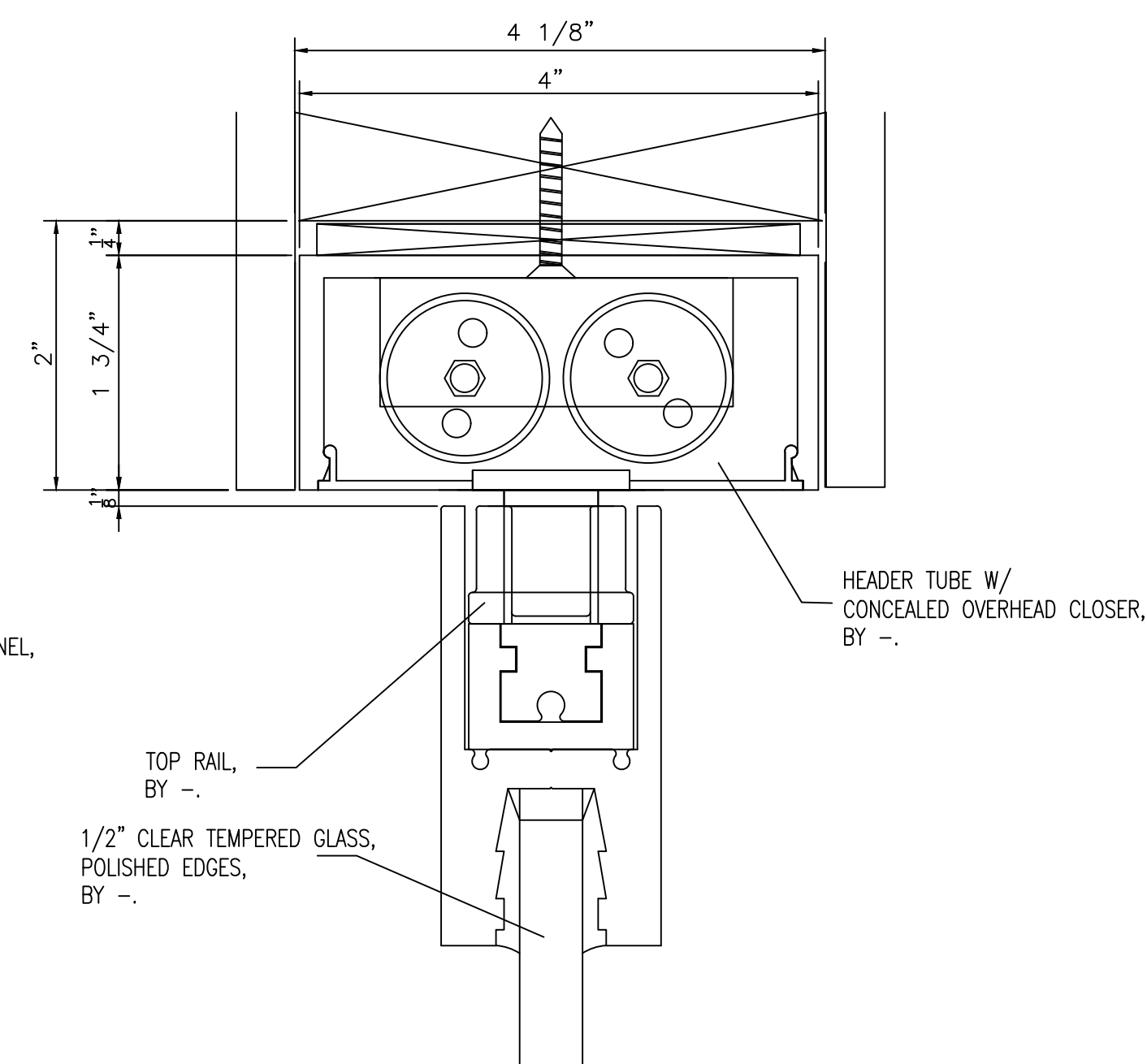
5 SECTION CUT ● SWING DOOR
