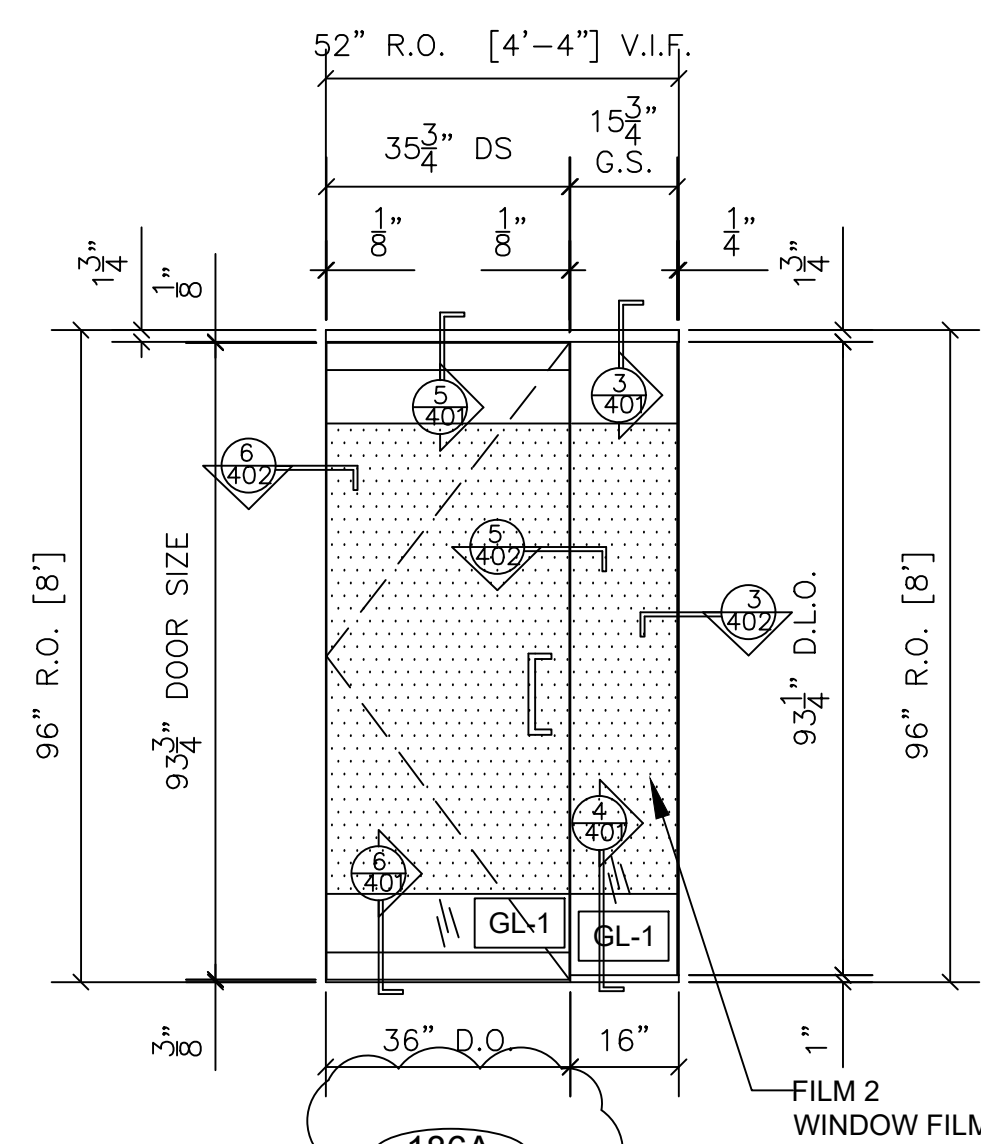
24 SWINGING DOOR SYSTEM FRAME ELEVATION SWINGING DOOR WITH RAILS AND SIDELITE ARCH. REF.: 1/A2.01 QTY LOCATION 1 BRAKE ROOM 186 1 TOTAL
