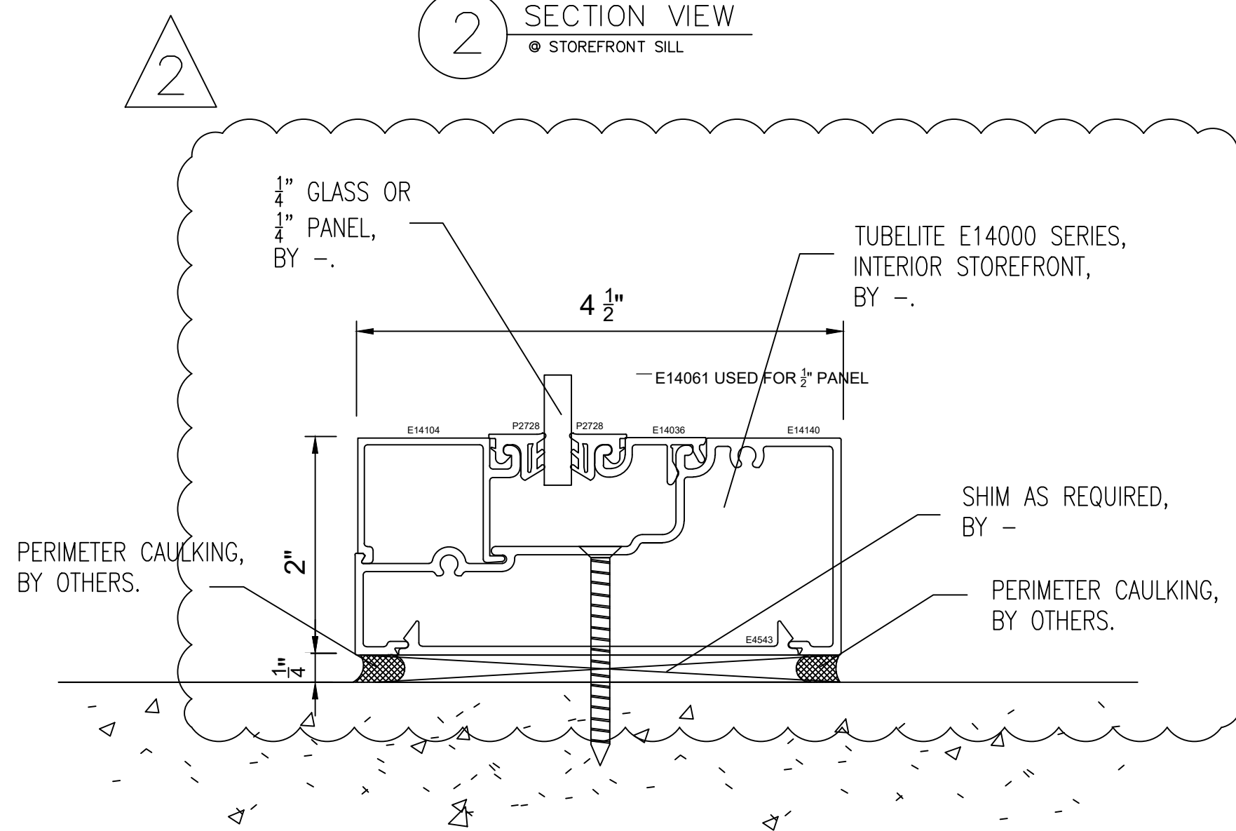
2A SECTION VIEW ● STOREFRONT SILL
