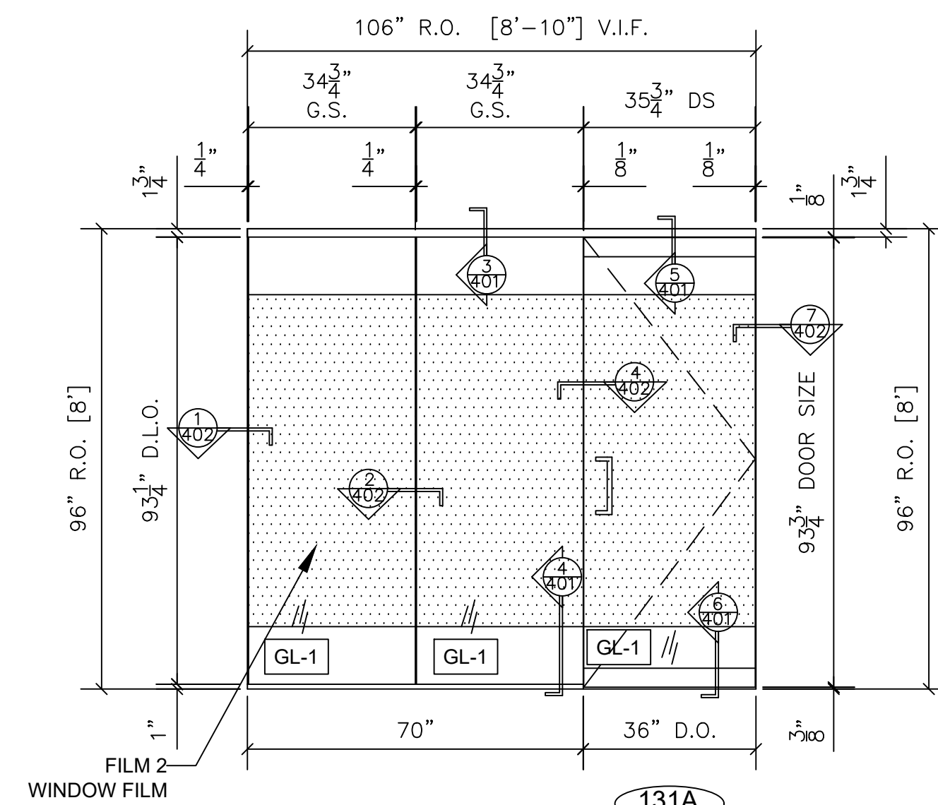
26 SLIDING DOOR SYSTEM FRAME ELEVATION CRL 70 SLIDING DOOR UNIT W/ SIDELITES ARCH. REF.: 1/A2.01 QTY LOCATION 1 METALS OFFICE 104 1 TOTAL
