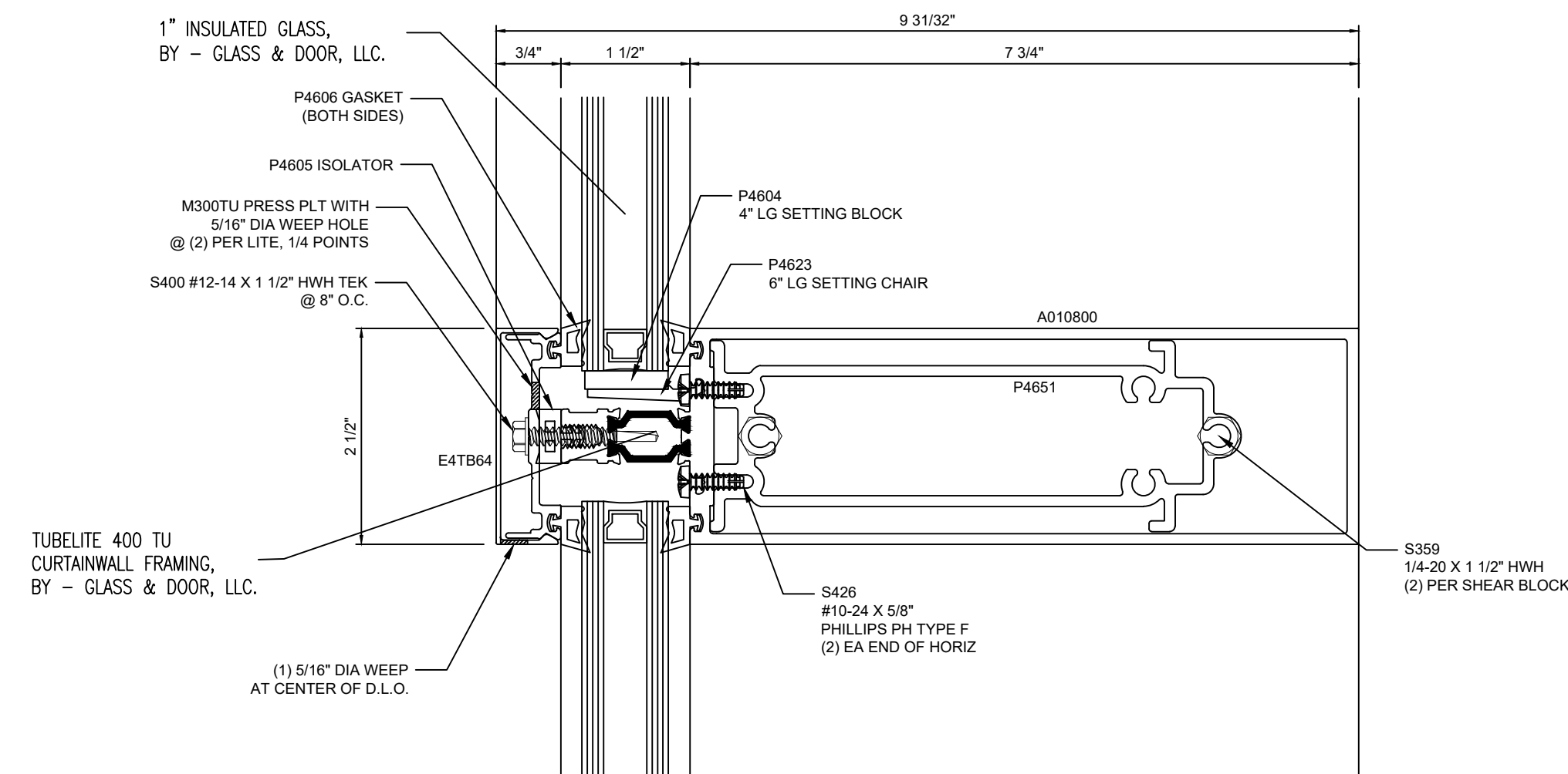
2 SECTION VIEW ● CURTAINWALL HORIZONTAL
