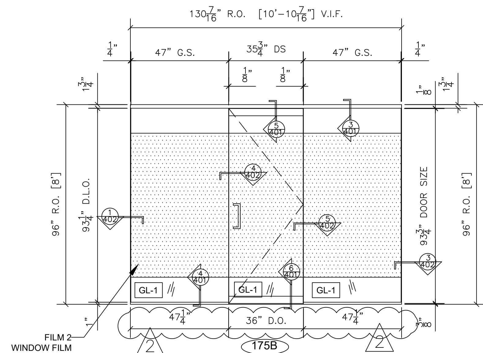
19 SWINGING DOOR SYSTEM FRAME ELEVATION SWINGING DOOR WITH RAILS AND SIDELITES ARCH. REF.: 1/A2.01 QTY LOCATION 1 VESTIBULE 175 1 TOTAL
