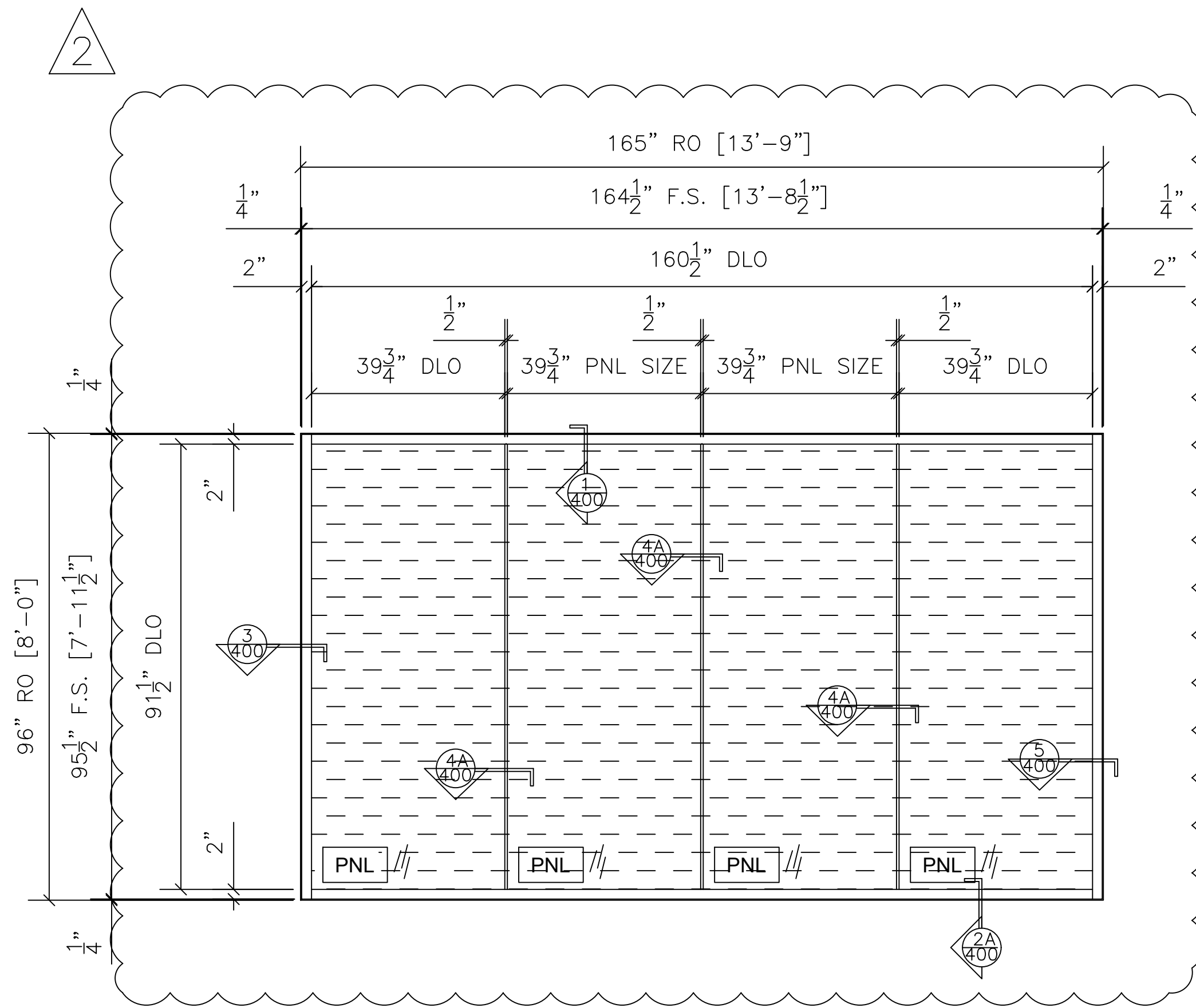
7A WINDOW TYPE 5 ELEVATION QTY LOCATION 1 HOLDING VESTIBULE 226 1 TOTAL TUBELITE E14000 INTERIOR STOREFRONT ARCH. REF.: 8/A3.31
