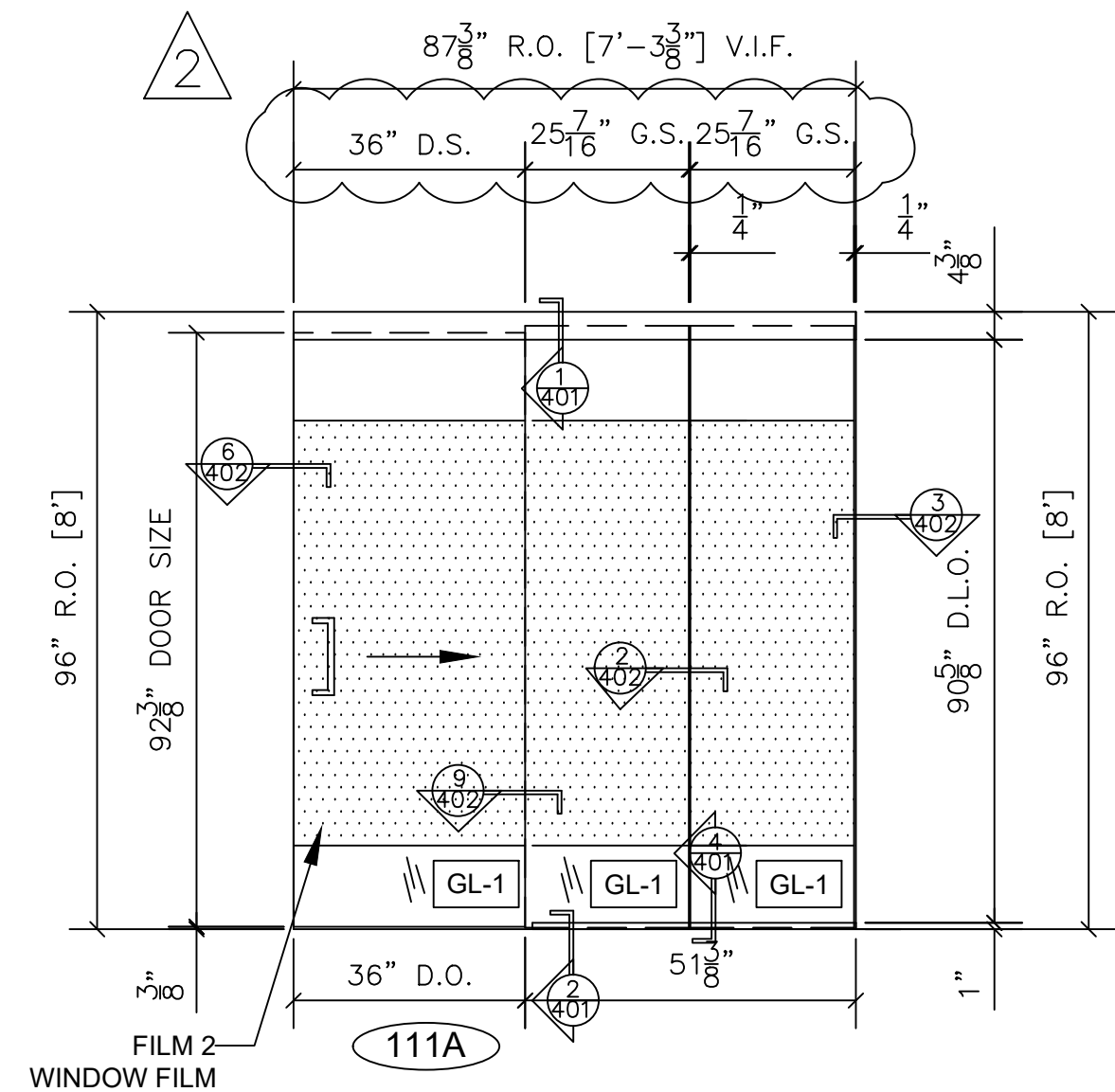
21 SLIDING DOOR SYSTEM FRAME ELEVATION CRL 70 SLIDING DOOR UNIT W/ SIDELITES ARCH. REF.: 1/A2.01 QTY LOCATION 1 HUDDLE/PHONE ROOM 111 1 TOTAL
