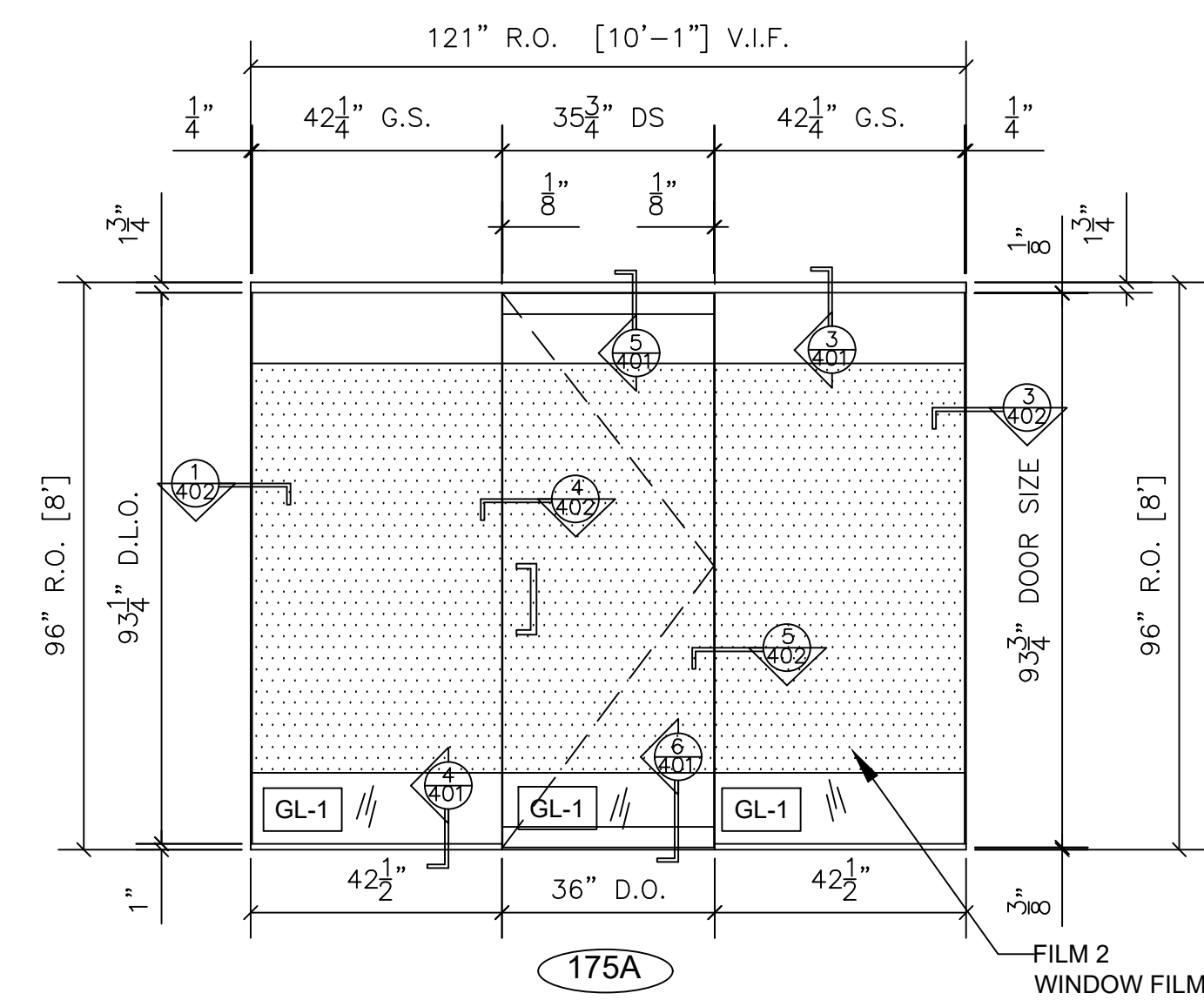
18 SWINGING DOOR SYSTEM FRAME ELEVATION SWINGING DOOR WITH RAILS AND SIDELITES ARCH. REF.: 1/A2.01 QTY LOCATION 1 VESTIBULE 175 1 TOTAL
