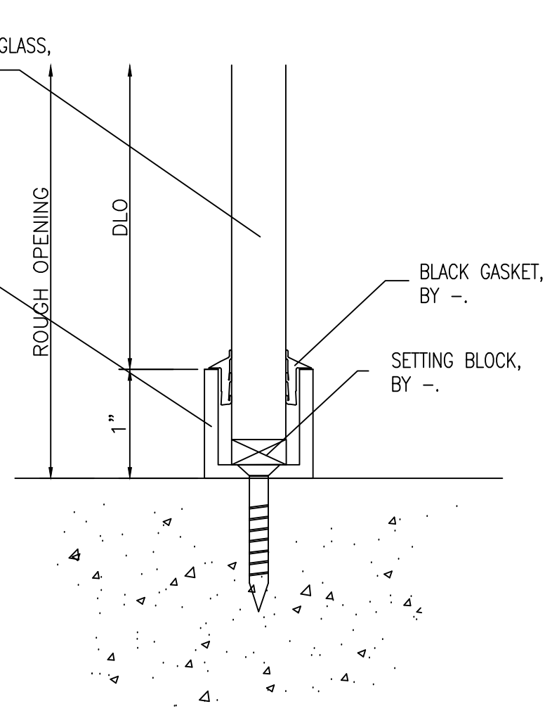
4 SECTION CUT ● SIDELITE BOTTOM CHANNEL
