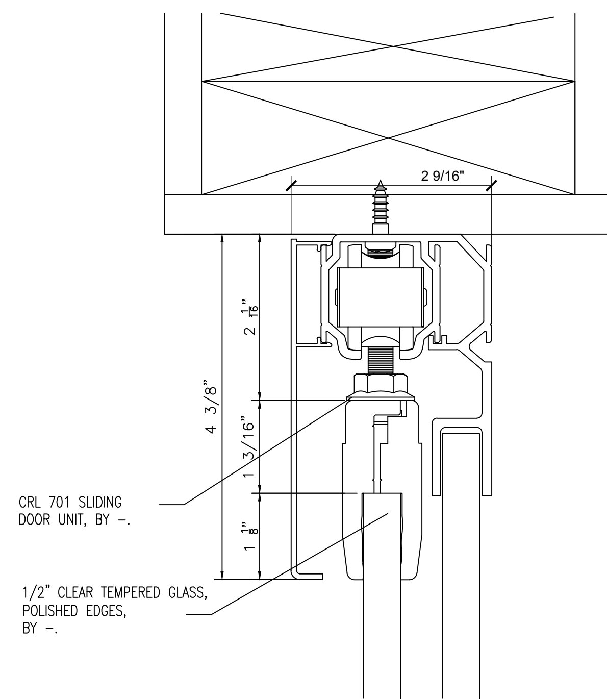
1 SECTION CUT ● SLIDING DOOR
