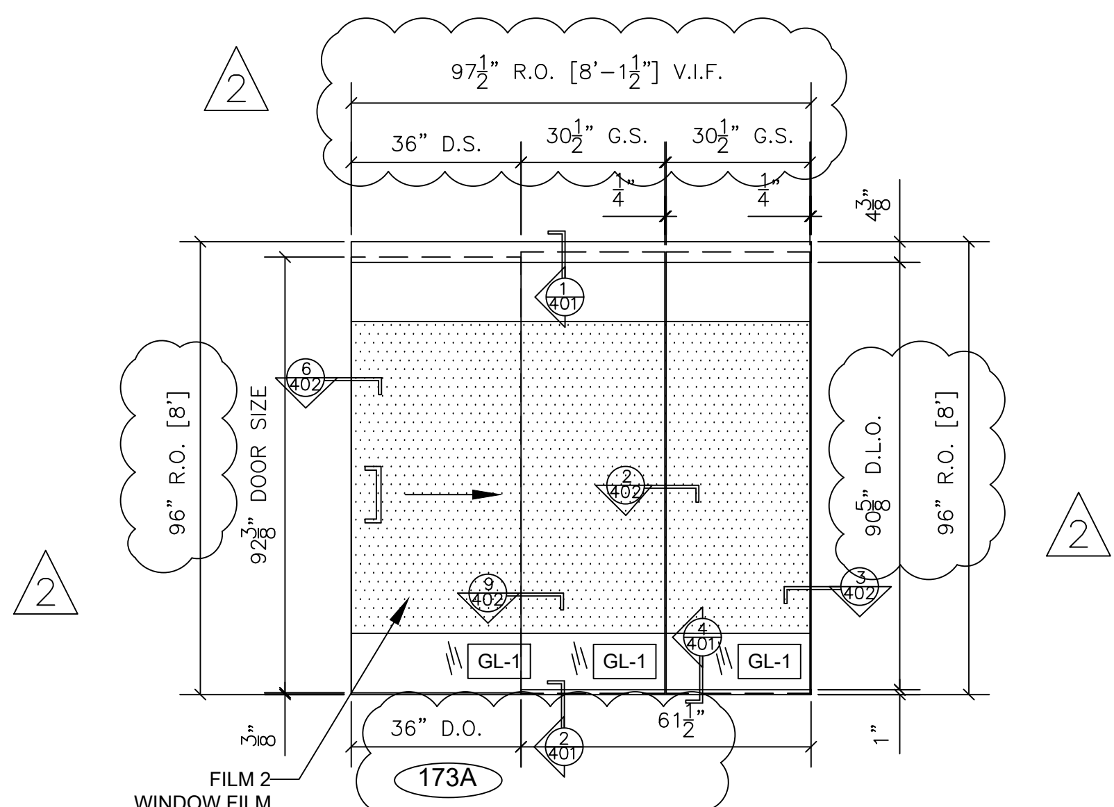
20 SLIDING DOOR SYSTEM FRAME ELEVATION CRL 70 SLIDING DOOR UNIT W/ SIDELITES ARCH. REF.: 1/A2.01 QTY LOCATION 1 HUDDLE/PHONE ROOM 173 1 TOTAL
