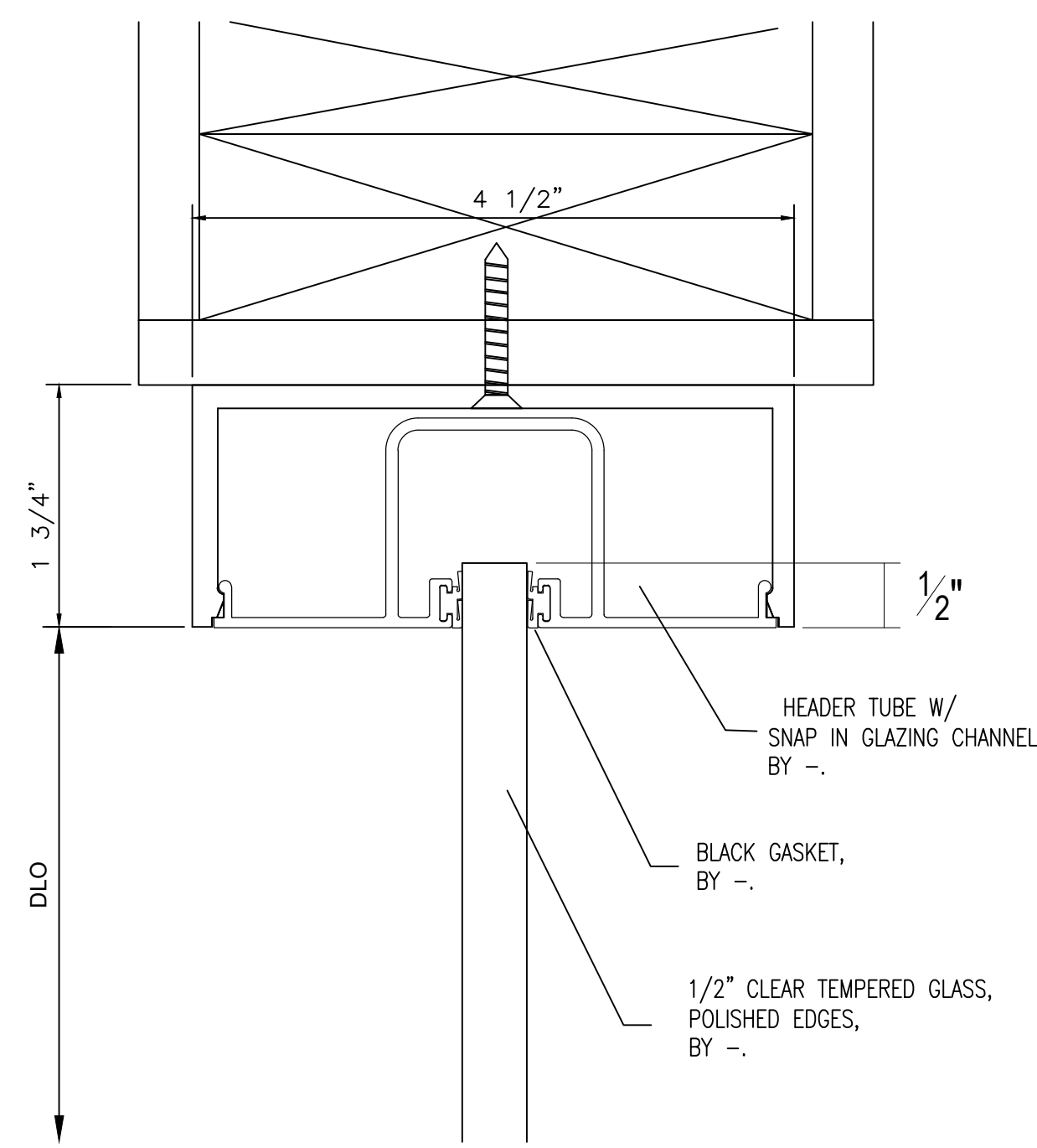
3 SECTION CUT ● SIDELITE HEADER
