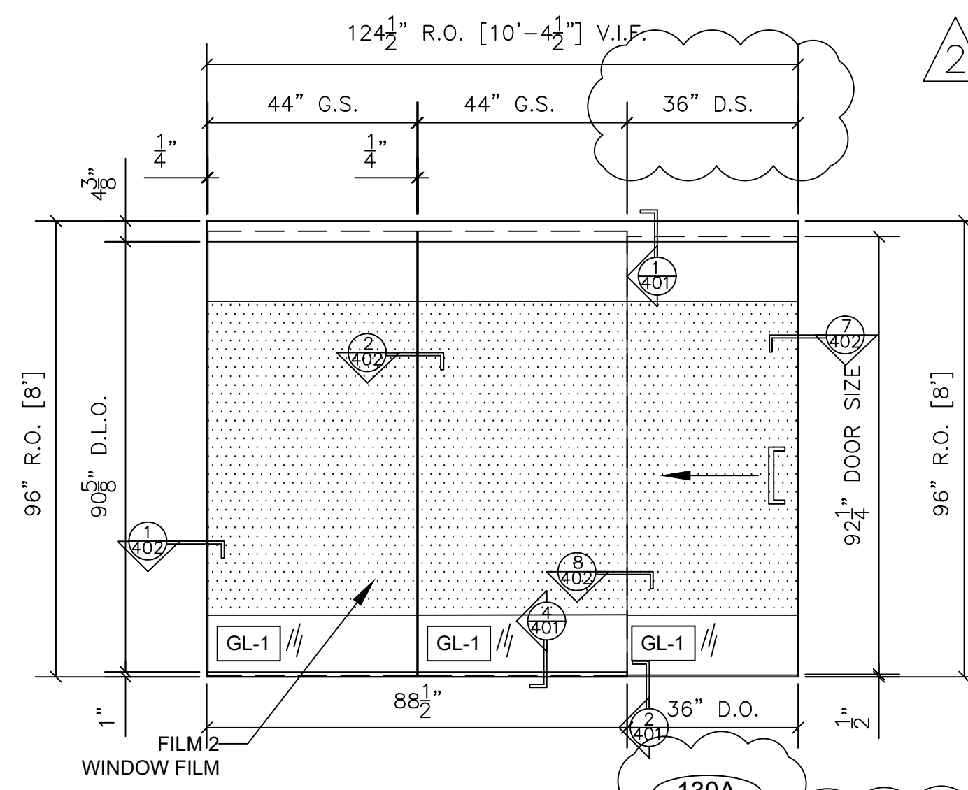
23 SLIDING DOOR SYSTEM FRAME ELEVATION CRL 70 SLIDING DOOR UNIT W/ SIDELITES ARCH. REF.: 1/A2.01 QTY LOCATION 1 API DIETARY SUPP 130 1 TOTAL
