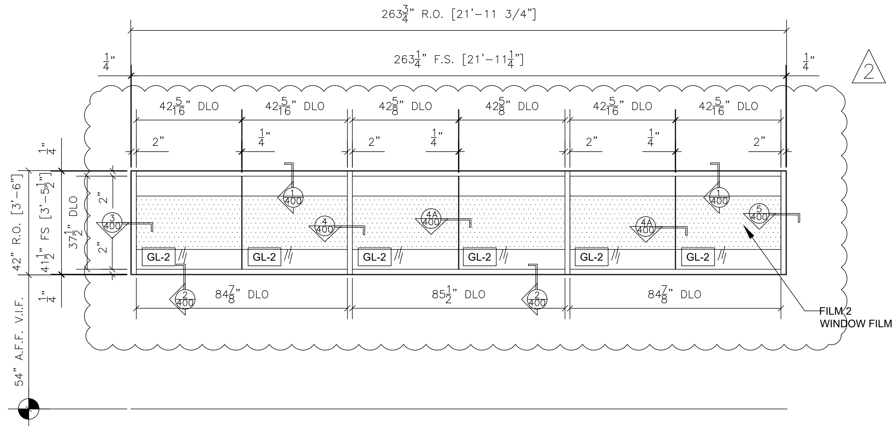
7 WINDOW FRAMING ELEVATION QTY LOCATION 1 NORTH ARTERY 123 1 TOTAL TUBELITE E14000 INTERIOR STOREFRONT ARCH. REF.: SIM. 4/A3.31
