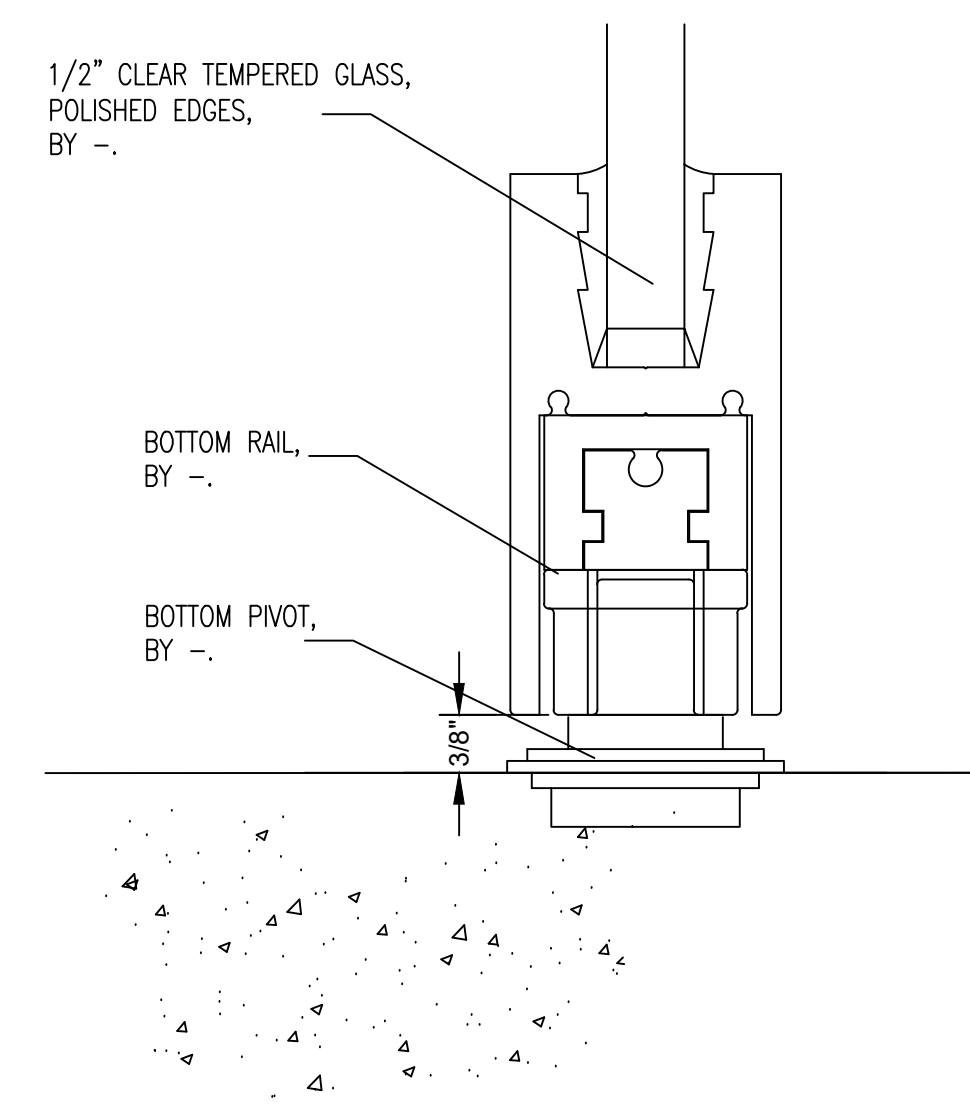
6 SECTION CUT ● SWING DOOR
