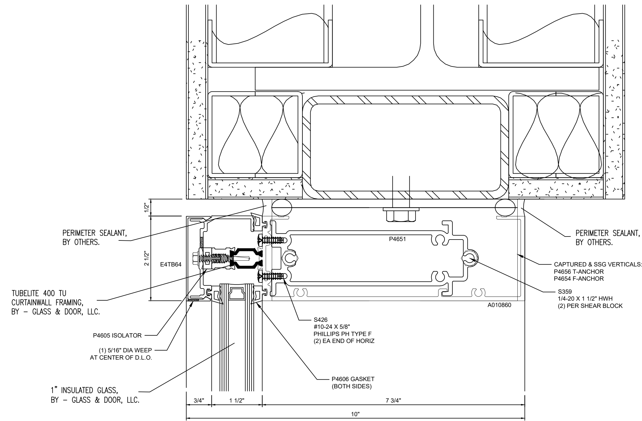
1 SECTION VIEW ● CURTAINWALL HEAD
