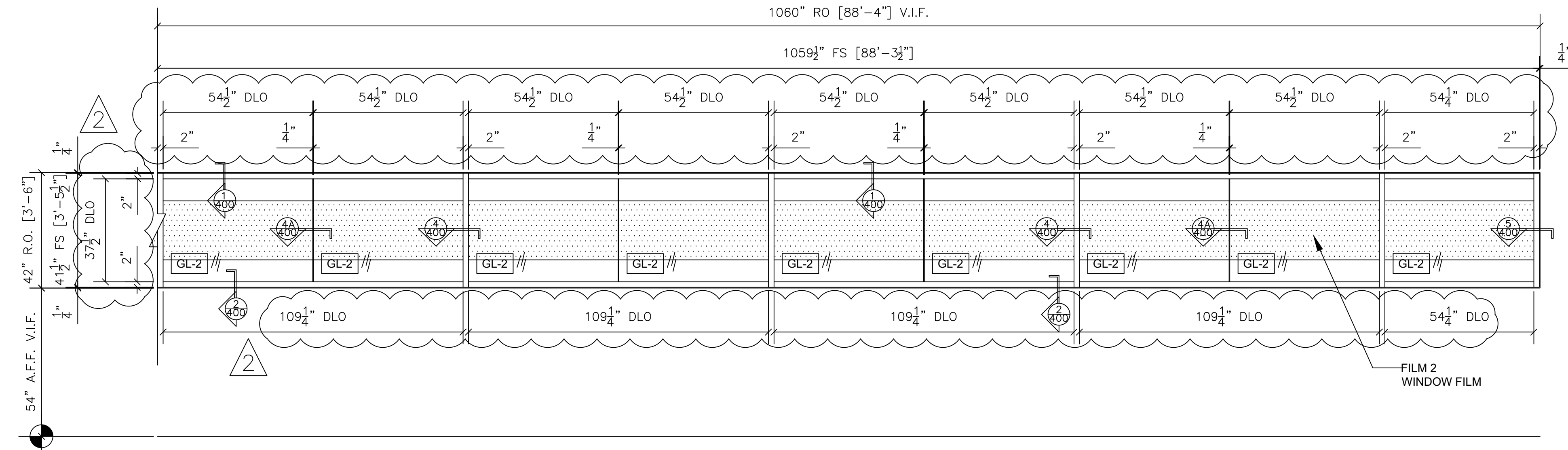
8 WINDOW FRAMING ELEVATION TUBELITE E14000 INTERIOR STOREFRONT ARCH. REF.: SIM. 4/A3.31 QTY LOCATION 1 SOUTH ARTERY 155 1 TOTAL
