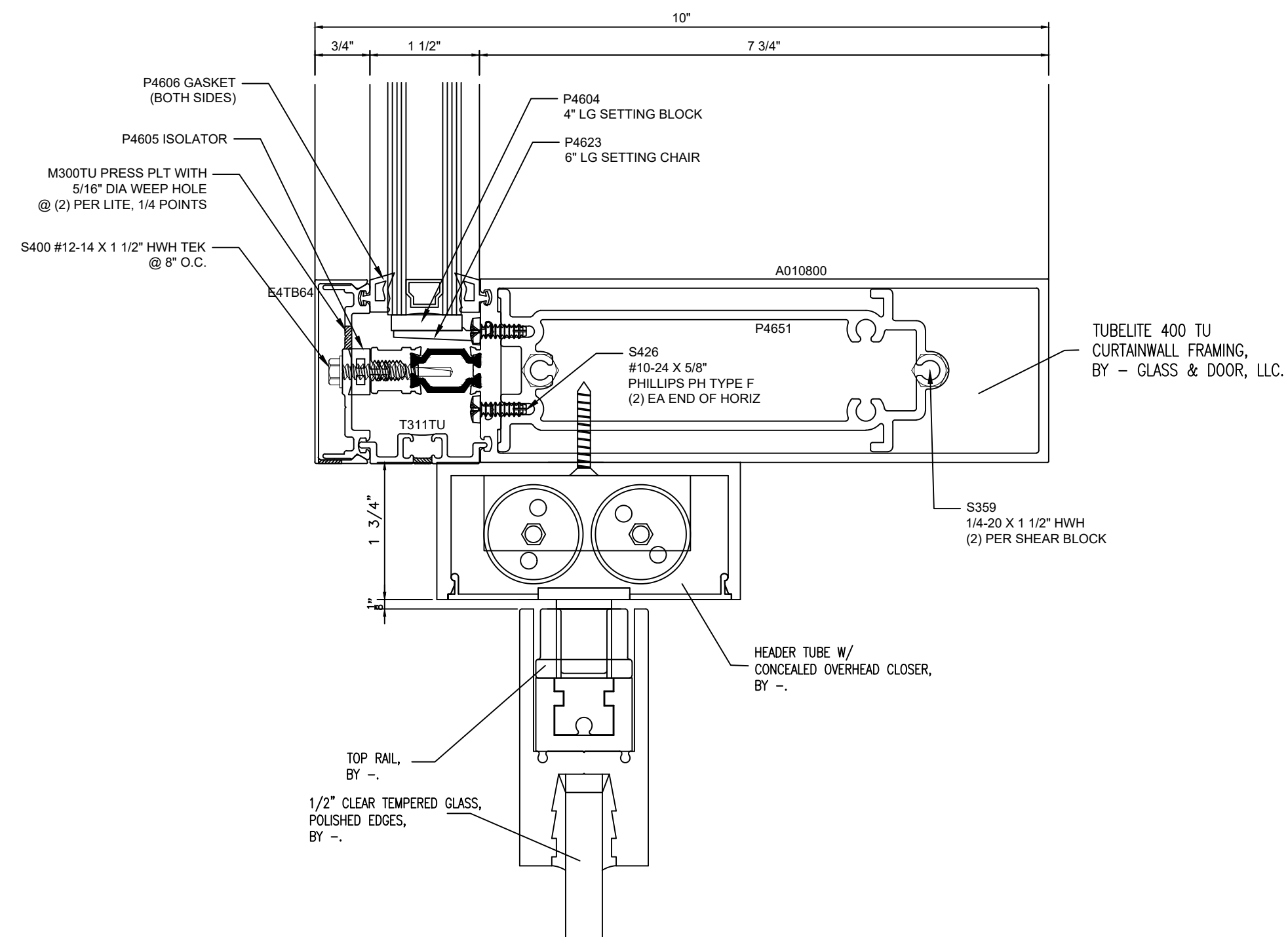
4 SECTION CUT ● GLASS DOOR TOP RAIL
